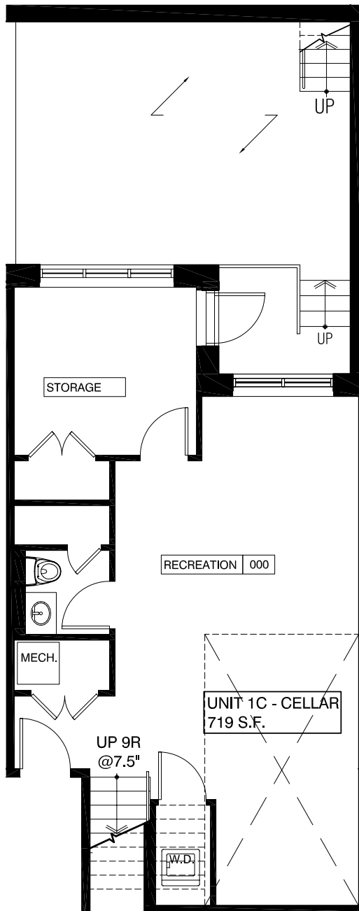
CELLAR
